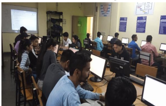
Python Programming
